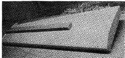
Sheeted wing panels are sanded with a long, straight sanding block. The important thing here is to get both halves as nearly identical as possible.
