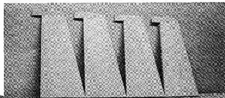
Four stabilizer blades, ready for joining. (The author builds these airplanes almost on a production line basis, which is why there are so many stabs.)
