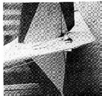
Tail surfaces use a clevis on a threaded rod for precise control throw adjustments.
