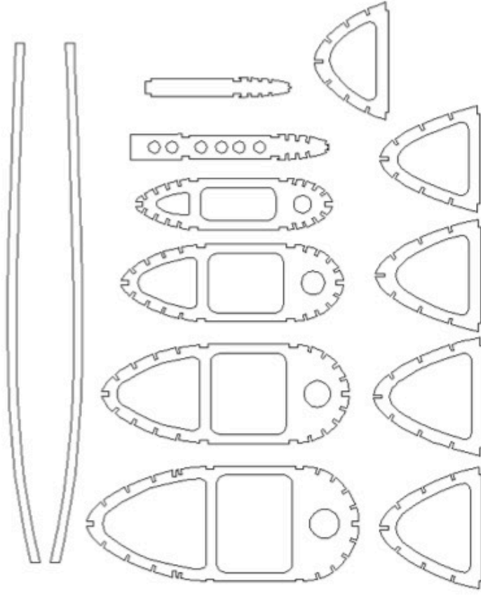
1/8" Balsa Formers
