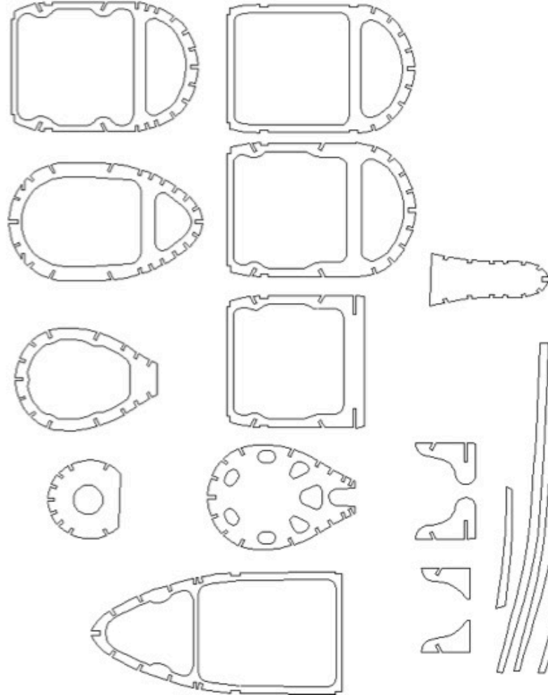
Lite Ply formers
