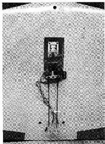
Servo installation in wing. Futaba S-20 used for allurers, S-8 for retract.
