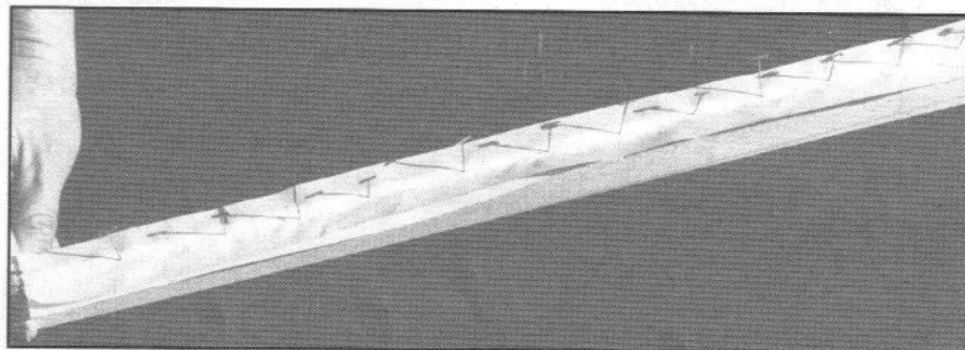
LEFT: Pin hinge to edge of control surface, be sure to keep stitch centered. RIGHT: Elevon pinned in place on wing, X-Hinge being ironed down.
